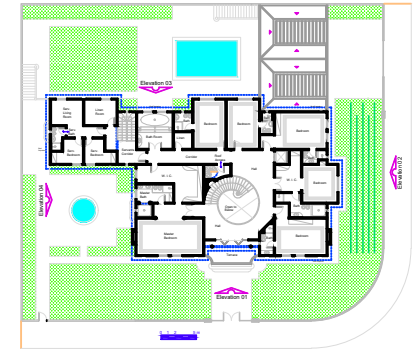
Second Floor Plan A = 392,63 m 2
