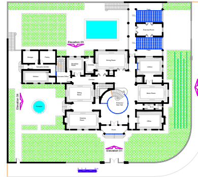
First Floor Plan A = 475,99 m 2
