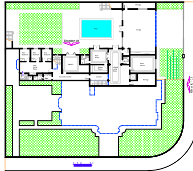
Lower Floor Plan A = 338,18 m 2
